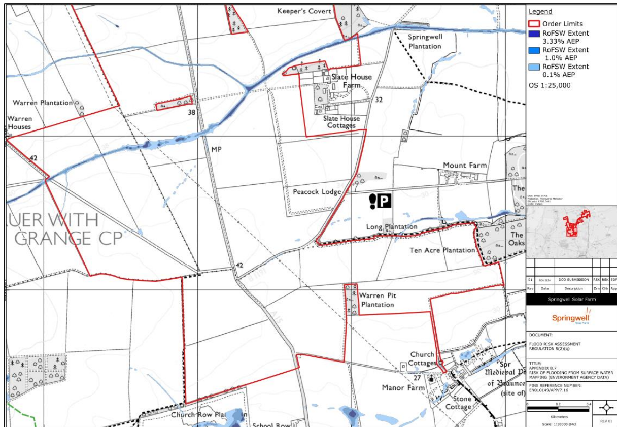
Plate 3.6: Surface water flood risk extents (1) (full map in Appendix B.7)
