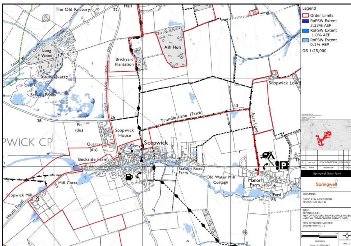
Plate 3.10: Surface water flood risk extents (5) (full map in Appendix B.11)
