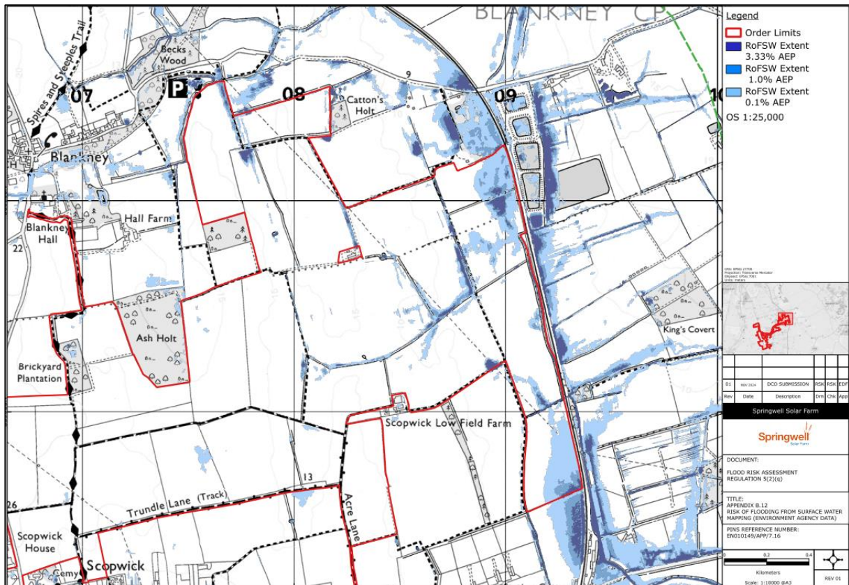
Plate 3.11: Surface water flood risk extents (6) (full map in Appendix B.12)
