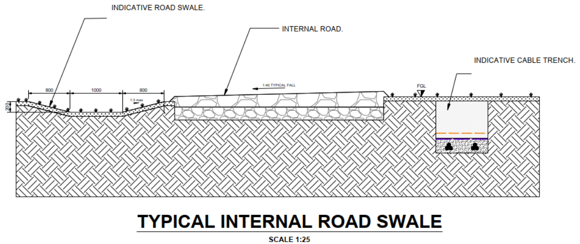
Figure 5 Typical access road section
