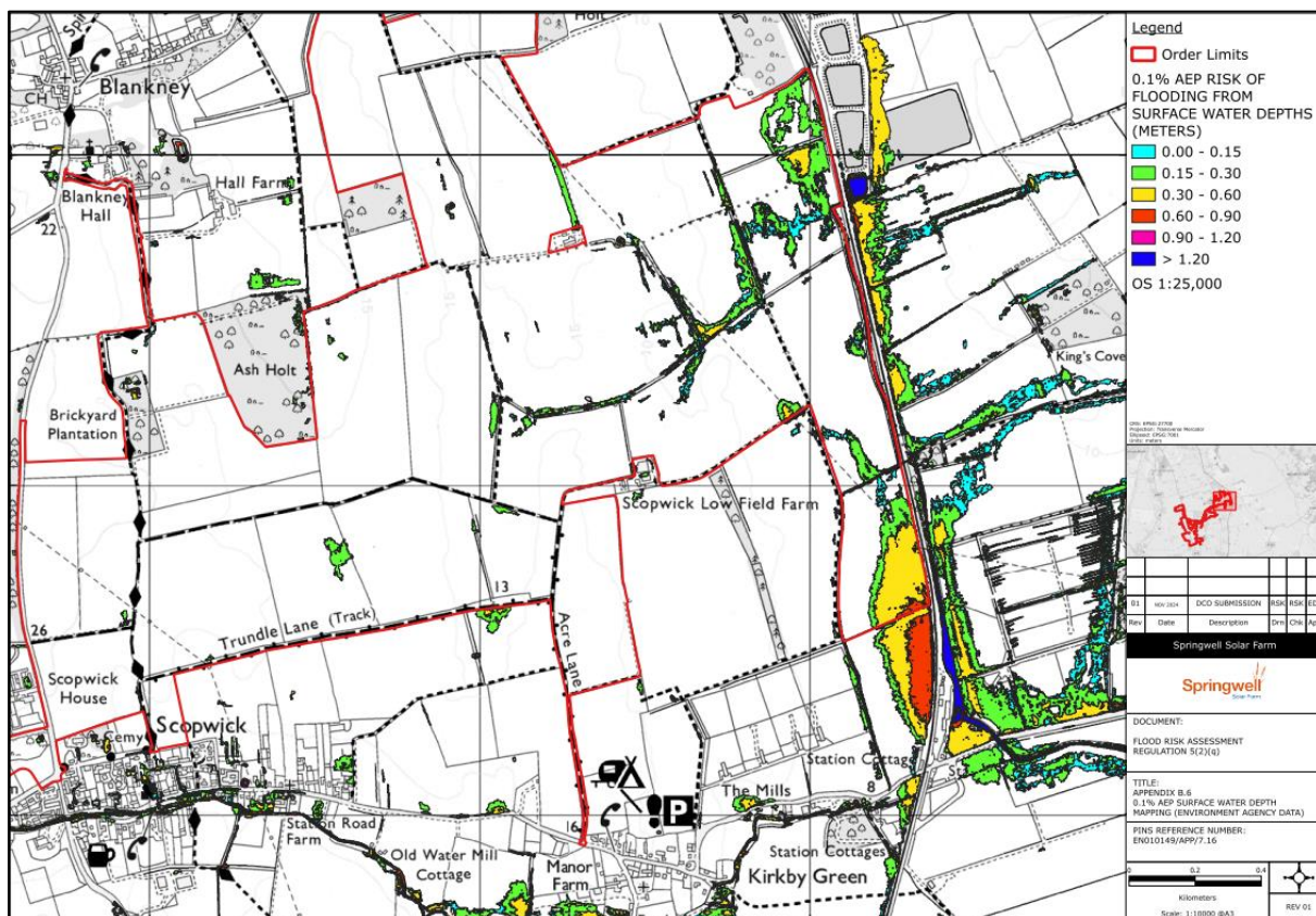
Plate 3.5: Surface water flood risk extents and depths for the 0.1% AEP modelled scenario. (full map in Appendix B.6)
