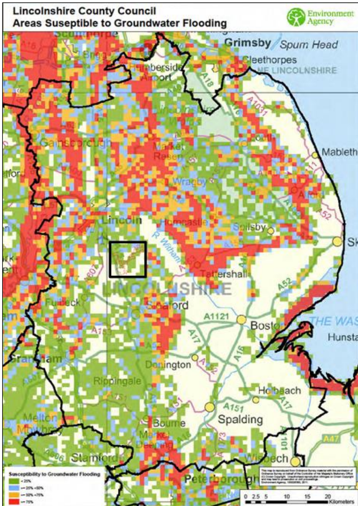
Plate 3.13: Lincolnshire County Council – Areas susceptible to groundwater flooding with approximate overlay of the Order Limits
