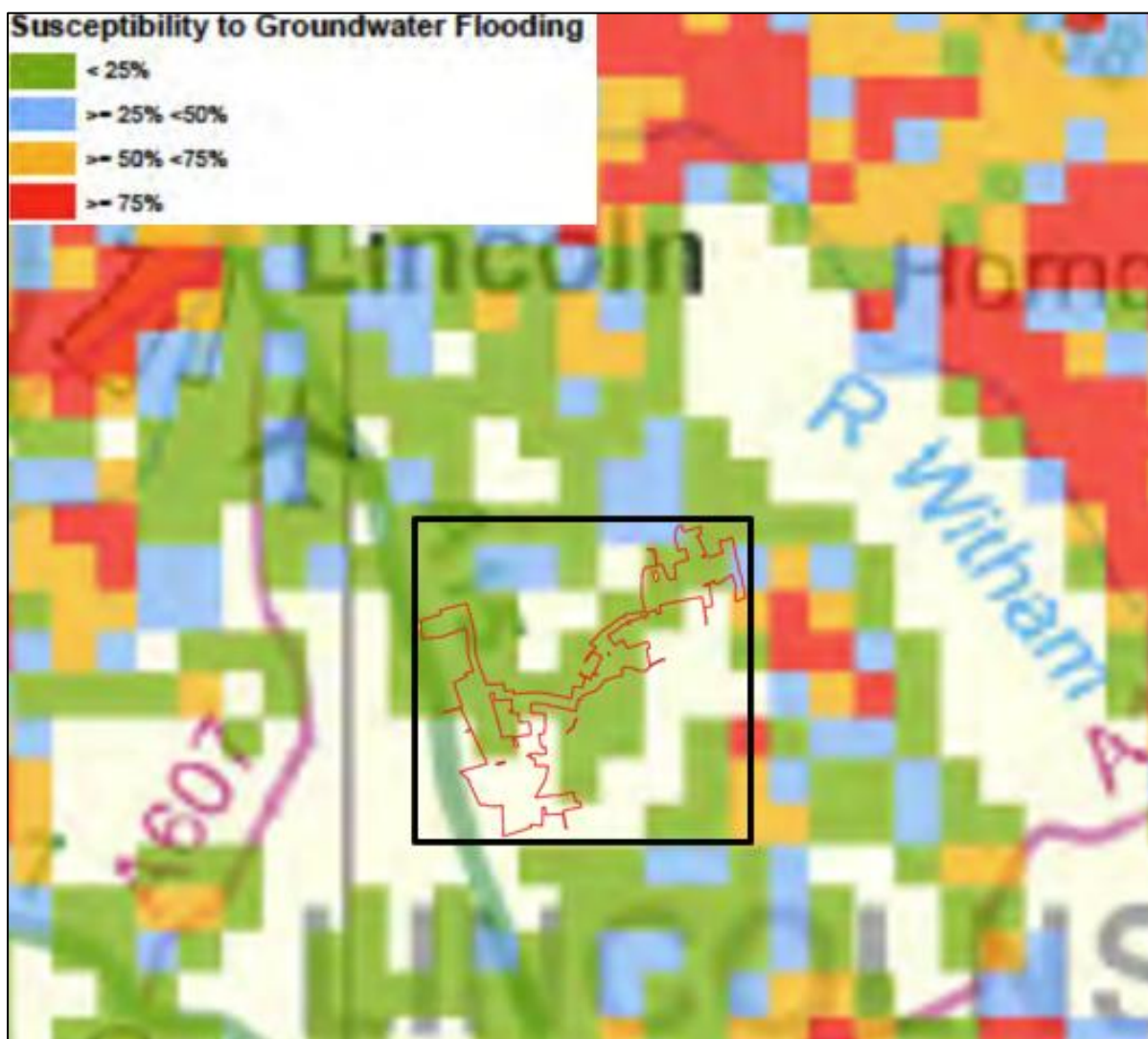
Plate 3.12: Lincolnshire County Council - Areas susceptible to groundwater flooding (close-up) with approximate overlay of the Order Limits
